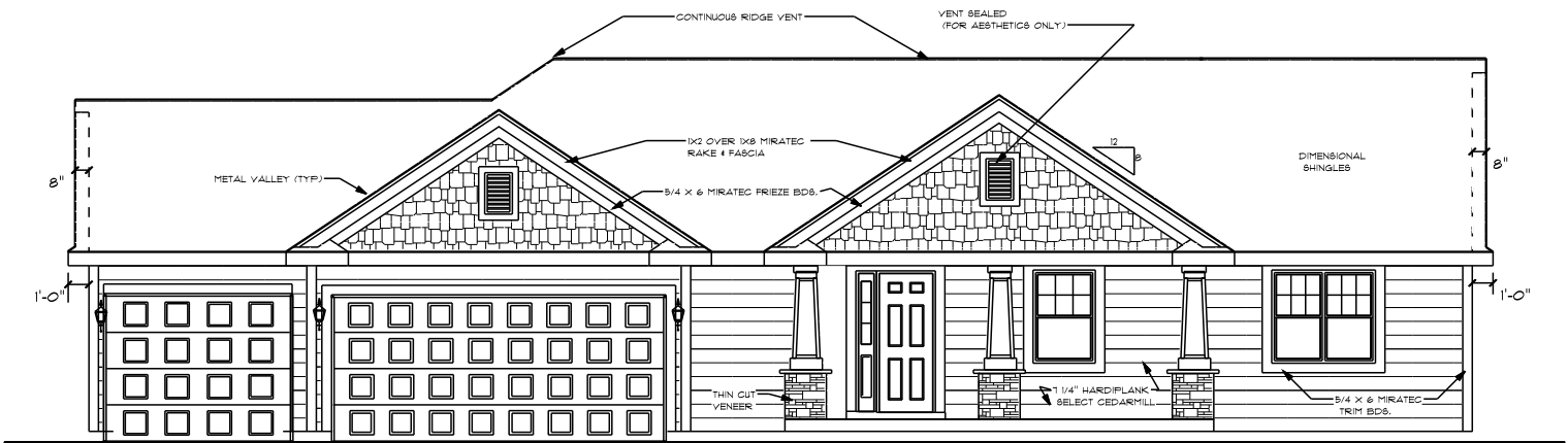
FRONT ELEVATION A
